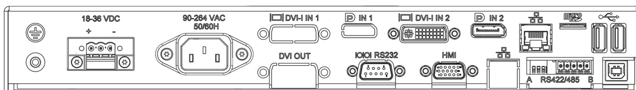
Figure: Terminal Plate for a full version Wave II Monitor (Newer version).
