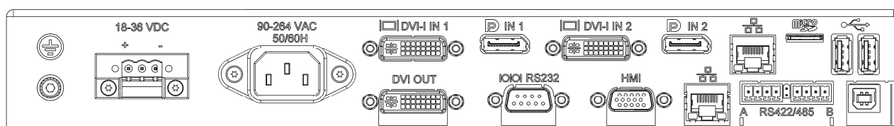
Figure: Terminal Plate for a full version Wave II Monitor.
